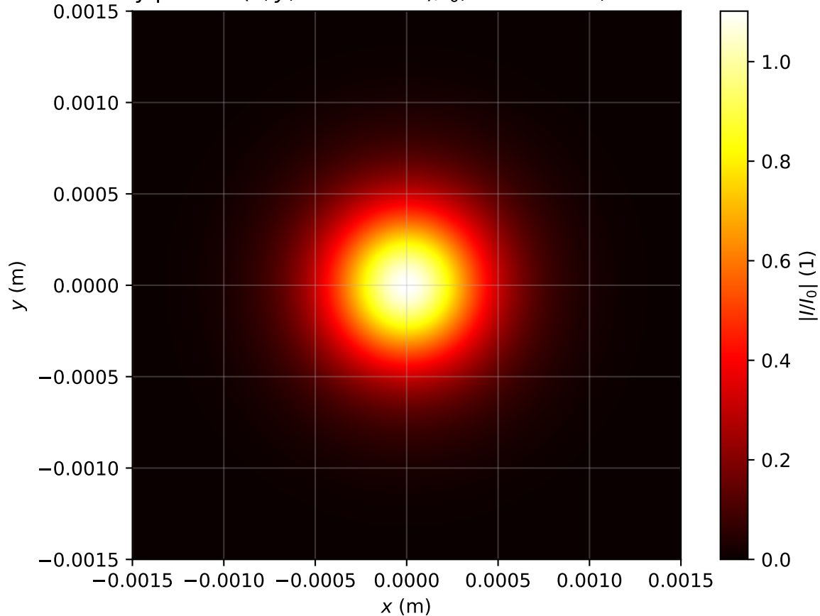
Intensity profile I(x, y, z = 1.274m)/I_0 , P_{in}=0.6P_{cr} , artificial time
